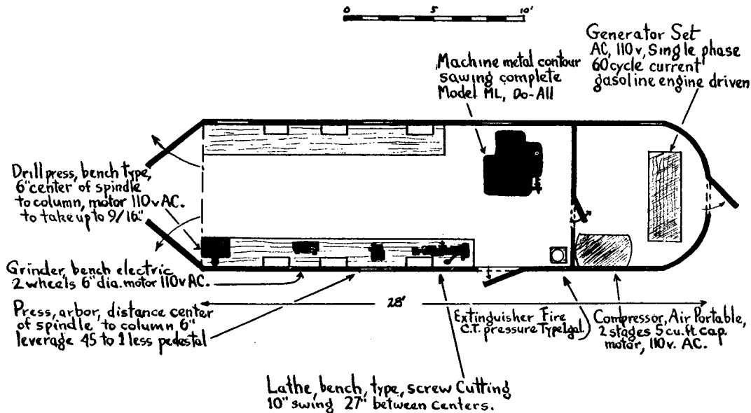
FIGURE 9.—Floor diagram of typical machine shop trailer.
