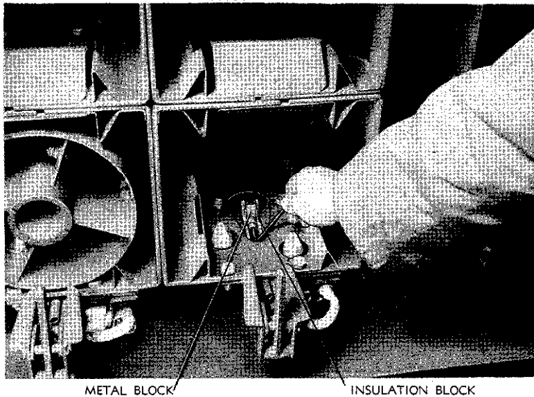
Figure 28—Replacement of Tail Latch Insulation Block
