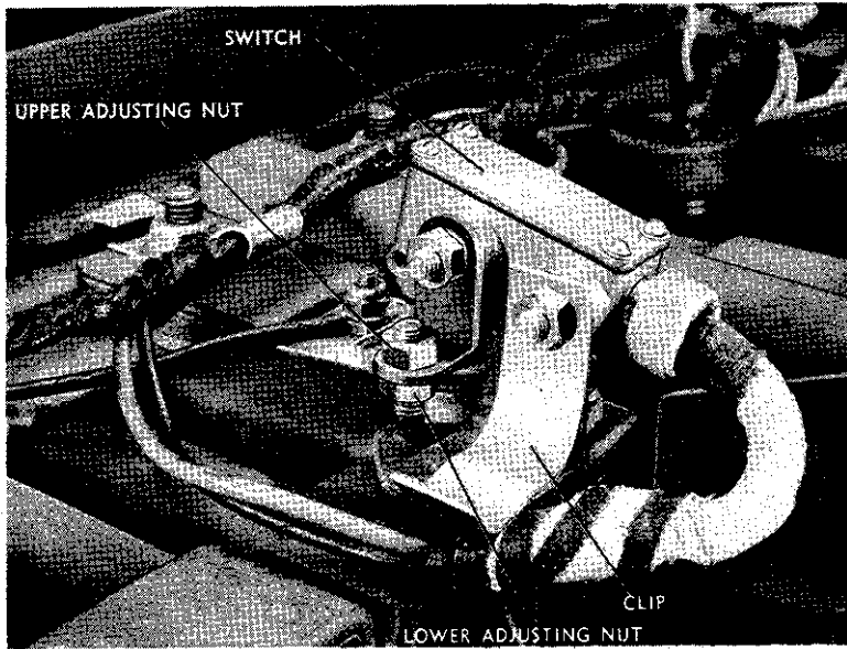
Figure 27—Adjusting Microswitch
